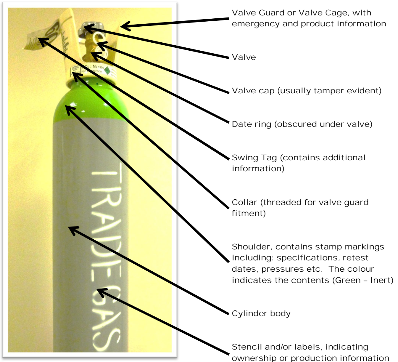
10 litre steel mixed gas beverage cylinder
